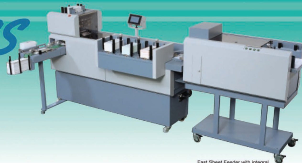
Fast Sheet Feeder with integral sheet accumulator and folding. Optical Mark Reading, OCR, Barcode and 2-D reading can be added. Jobs can be stored to simplify changeover.
